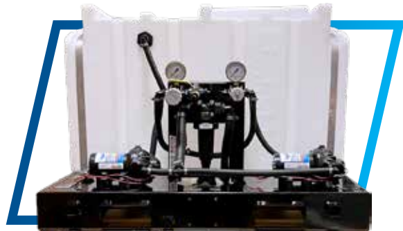
100 Gallon Low Profile Sprayer
